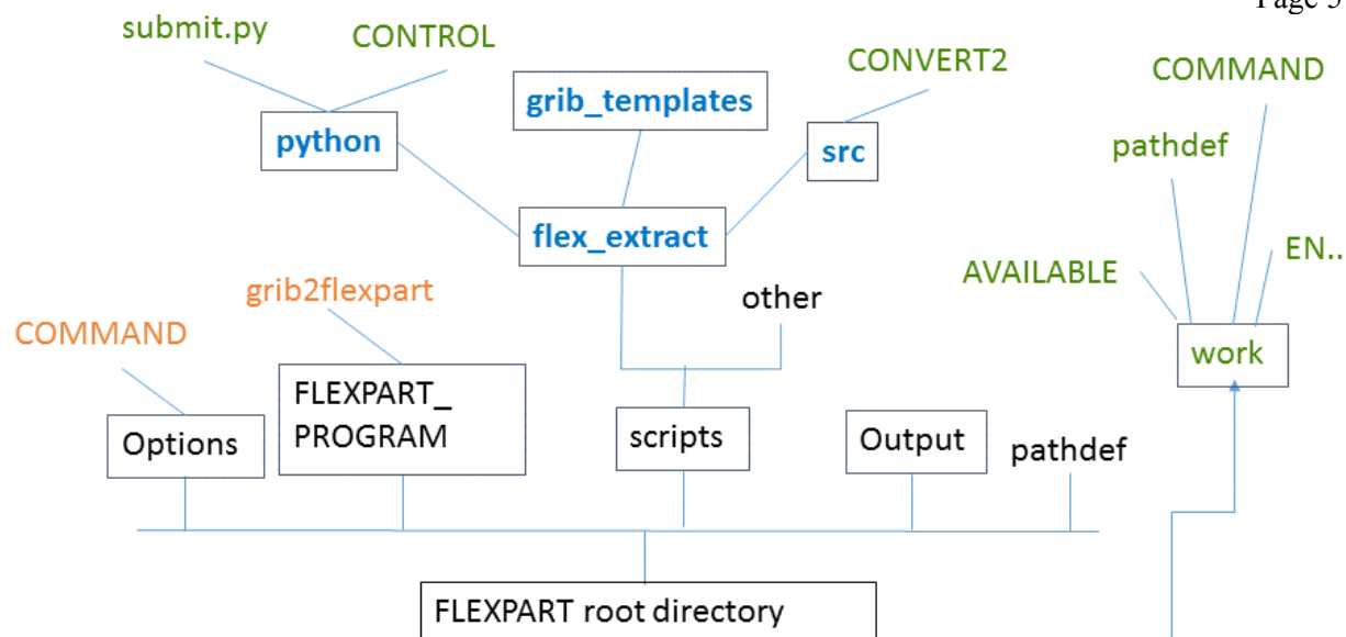
Fig. 1: FLEXPART directory structure (black) with directories in rectangles, files as text. Flex_extract software should reside in scripts directory. In order to create input files on height levels (fp files) flex_extract will need to have access to COMMAND file and grib2flexpart executable (red). Flex_extract software will create directory work and place all output files there. Usually the work directory will reside on a separate large file system.
